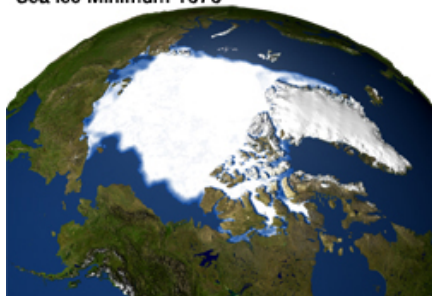
Sea Ice Minimum 1979
